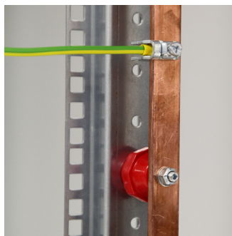
detailed view: earthing cable K2303.x installed at earthing bar K3930V42
